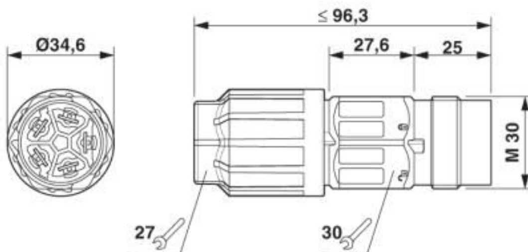
QPD C 5x2.5 dimensional drawing
