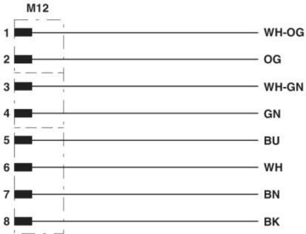
Circuit diagram
