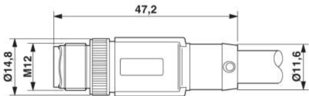
M12 connector, straight, shielded
