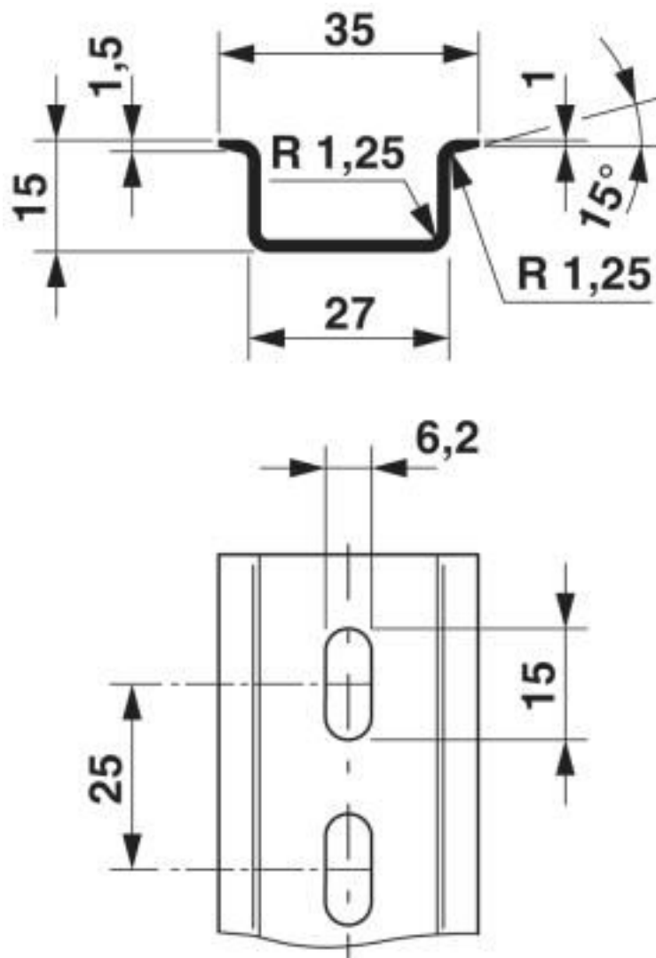
Dimensional drawing
