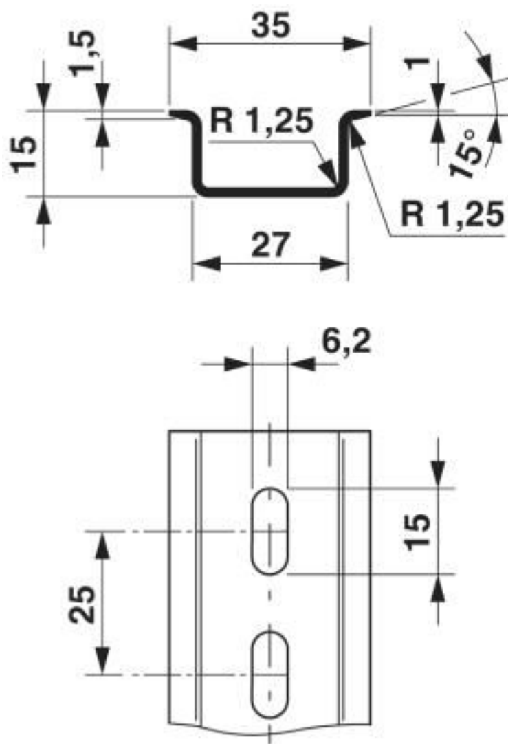
Dimensional drawing
