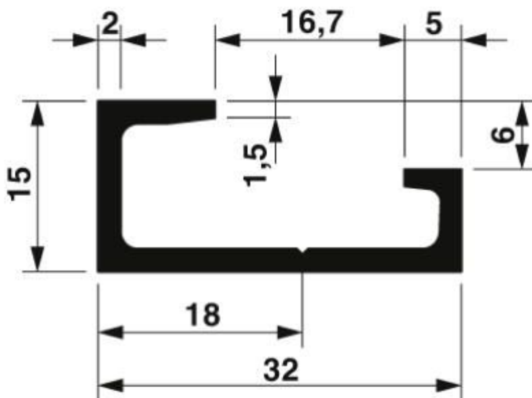
Dimensional drawing
