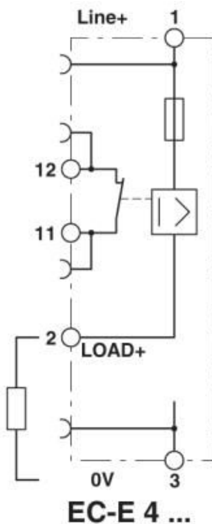
Circuit diagram
