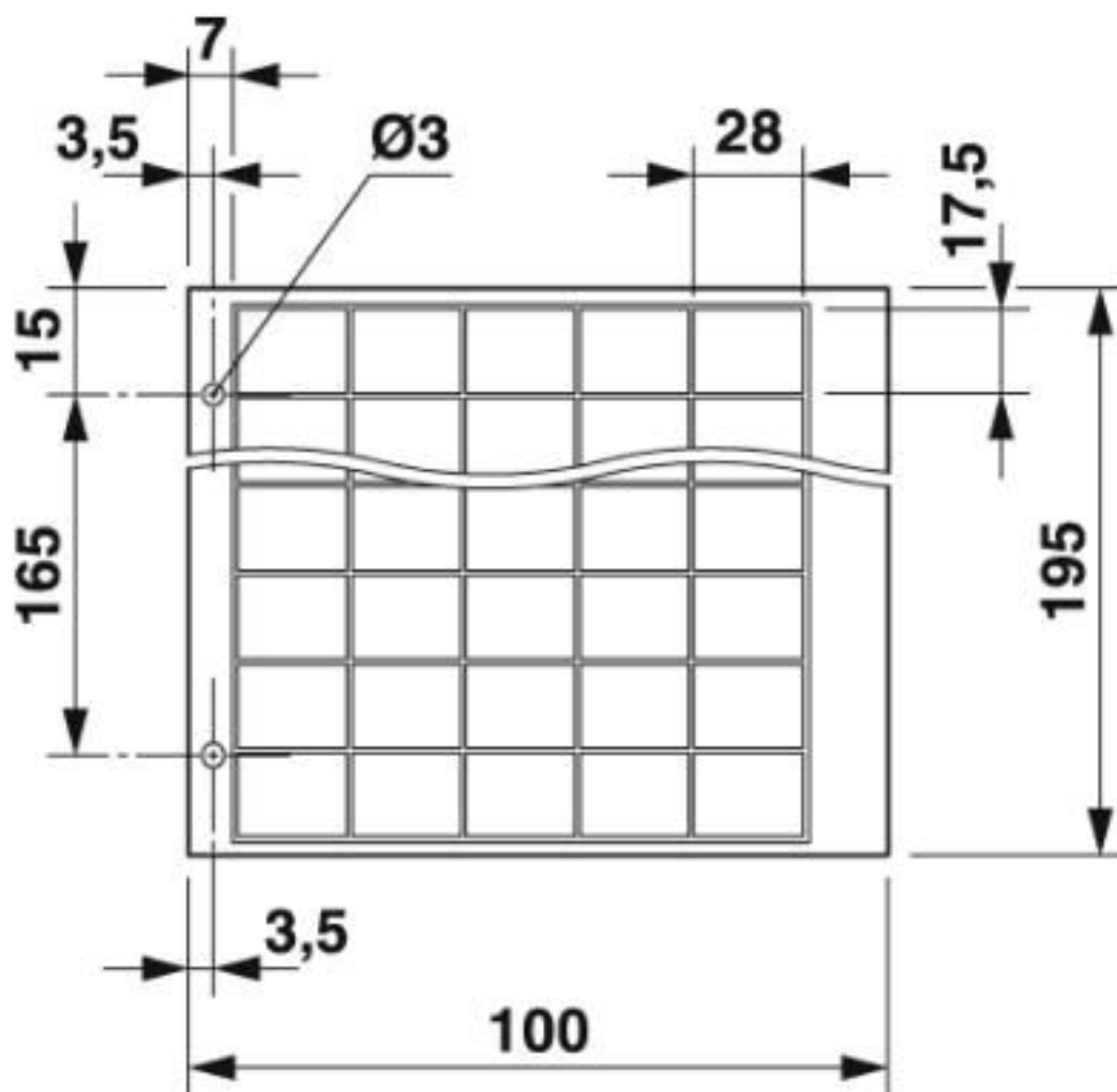
Dimensional drawing
