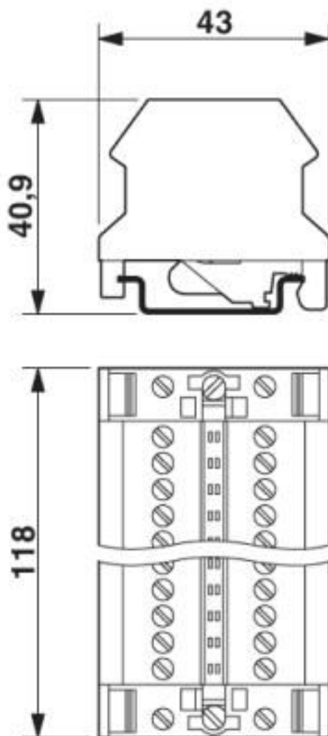
Dimensional drawing
