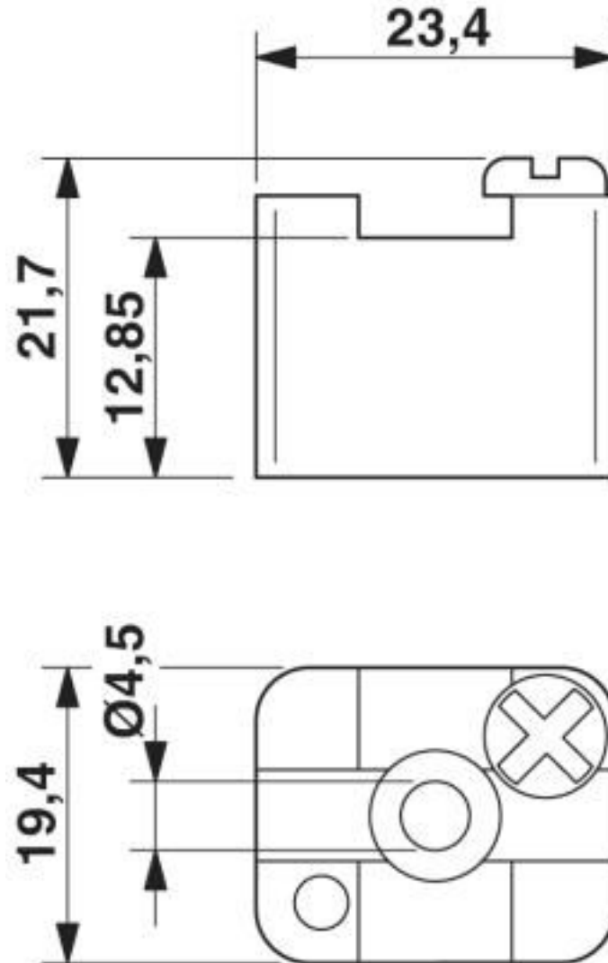
Dimensional drawing
