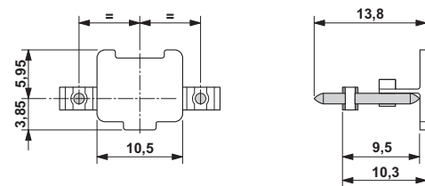
Pad position for PST 1,3/...5,0 R...
