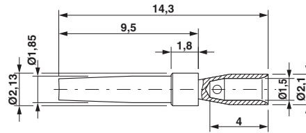
Dimensional drawing
