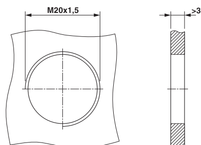
Installation dimensions
