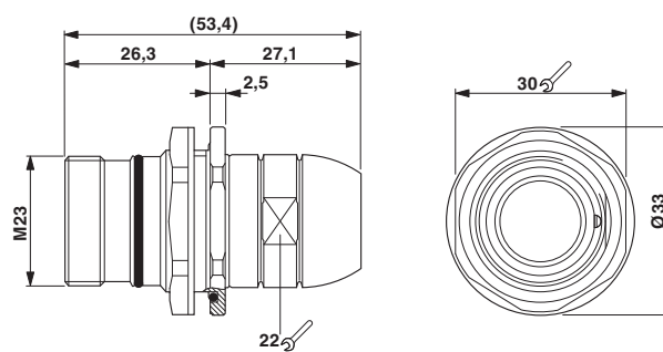
Dimensional drawing
