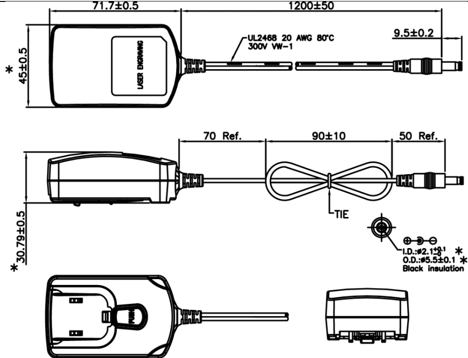
PSM10R-050A(M)-R: mm
