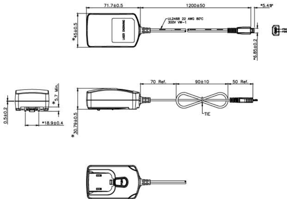
PSM10R-050A(M)-R: mm
