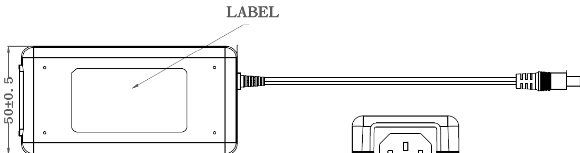
BOTTOM VIEW
