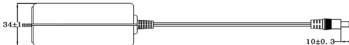
SIDE VIEW
