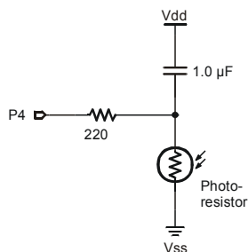
Figure 4.4 Circuit for use with rcTime
