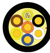
FSHRB12-06S12C 12 fiber Loose Tube with 6x12 AWG
