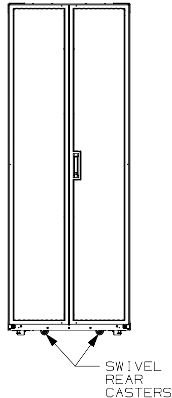
REAR VIEW
