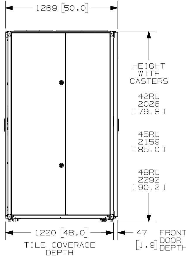
LEFT VIEW
