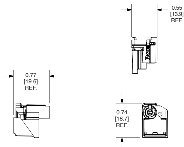
PSL-DCPLRE Recessed
