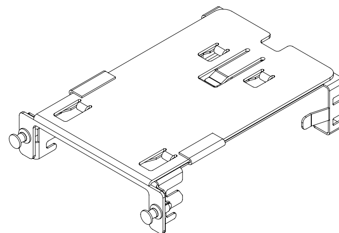
ISO VIEW
