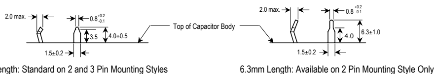
Pin Dimensions
