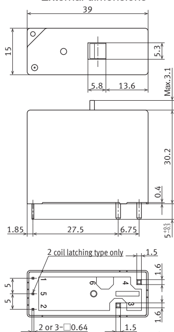
External dimensions
