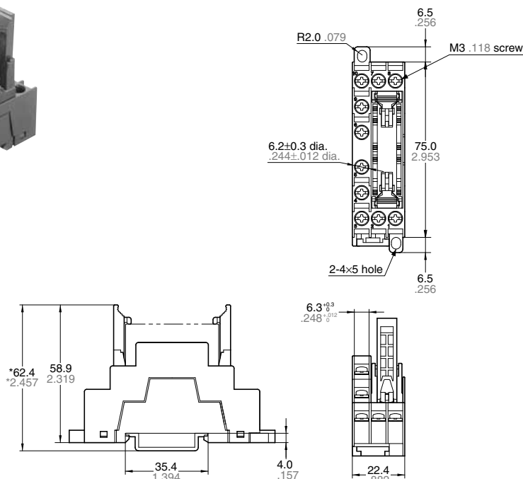
External dimensions
