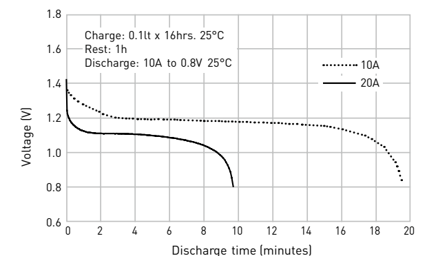
TYPICAL DISCHARGE CHARACTERISTICS
