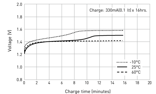
TYPICAL CHARGE CHARACTERISTICS
