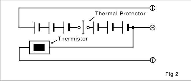
Basic pack configuration circuit
