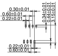
Recommended metal mask pattern Metal mask thickness: When 120μm (Front terminal portion opening area ratio: 96%) (Back terminal portion opening area ratio: 96%)
