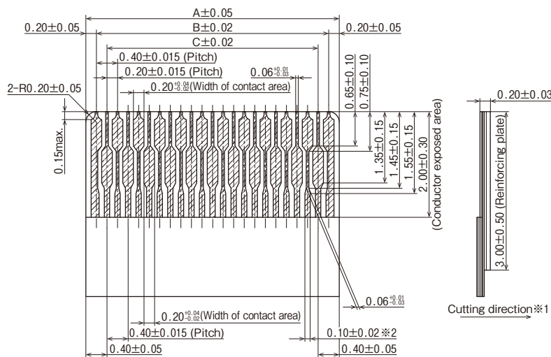
Dimension table
