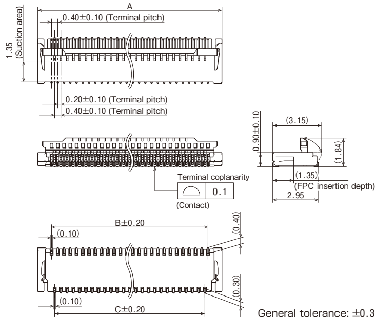
Dimension table
