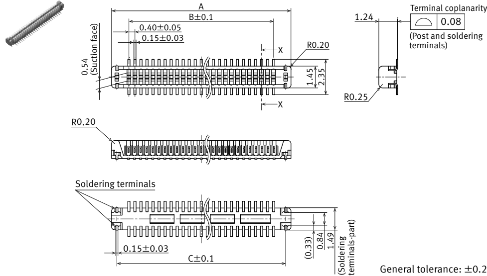
External dimensions
