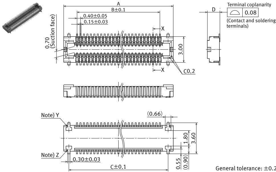
External dimensions
