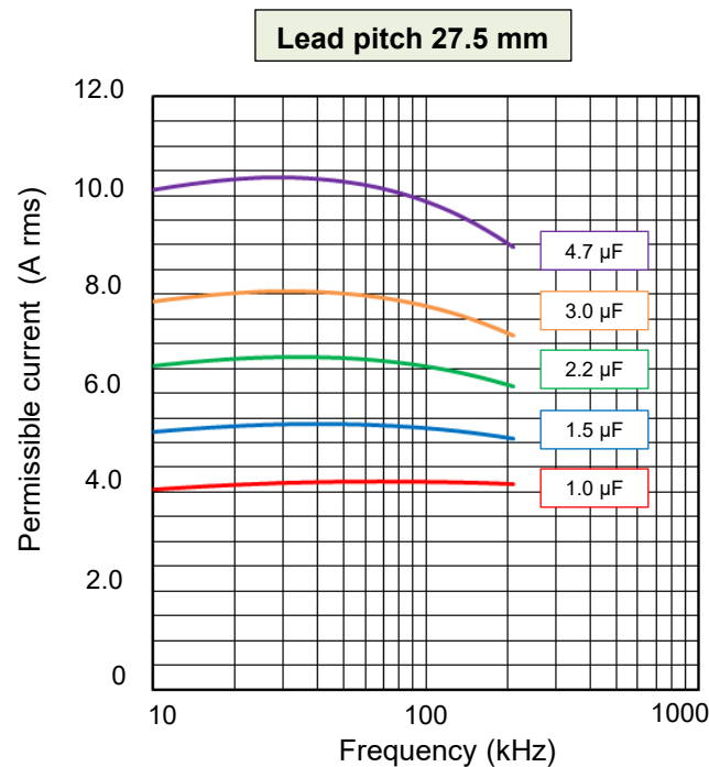
[ Permissible Current ]
