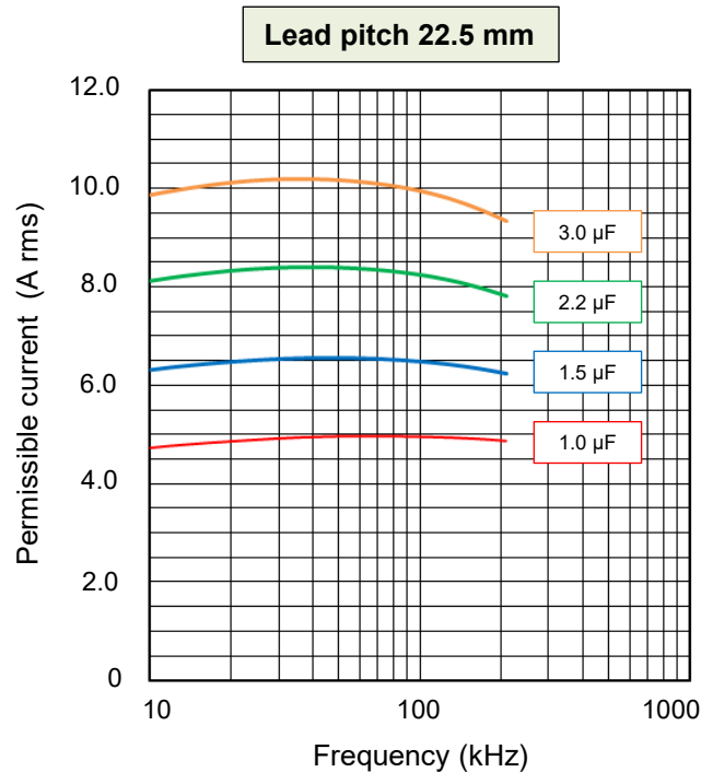
[ Permissible Current ]
