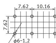
Recommended PC board pattern (BOTTOM VIEW)
