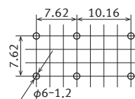
Recommended PC board pattern (BOTTOM VIEW)
