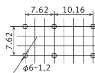
Recommended PC board pattern (BOTTOM VIEW)
