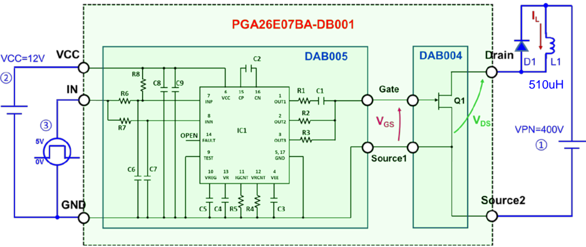
Figure 13: PGA26E07BA-DB001 in a simple chopper circuit
