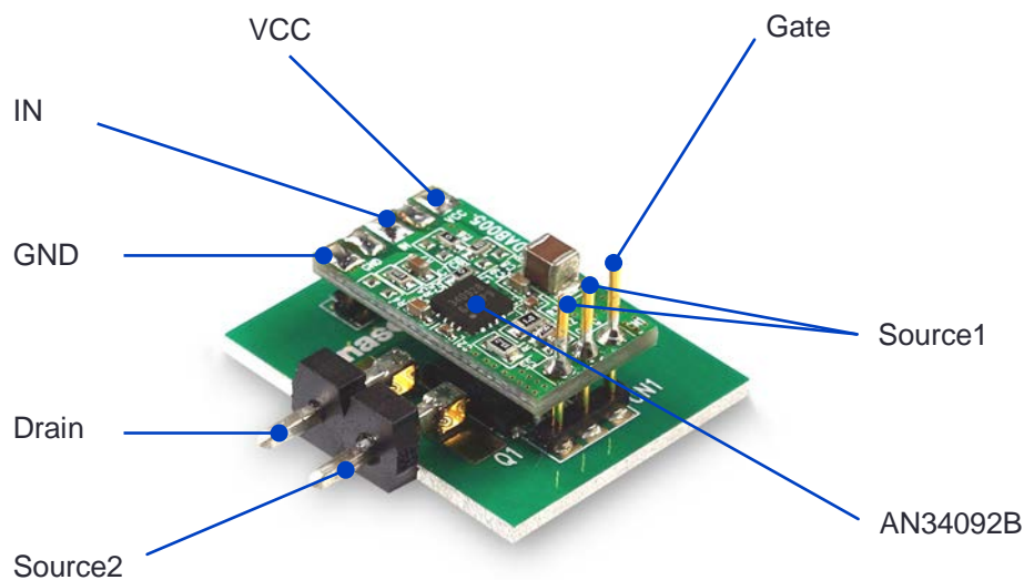
Figure 1: SMD to Thru-Hole Conversion Kit (PGA26E07BA-DB001)
