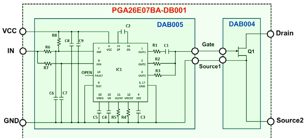
Figure 6: PGA26E07BA-DB001 Block diagram
