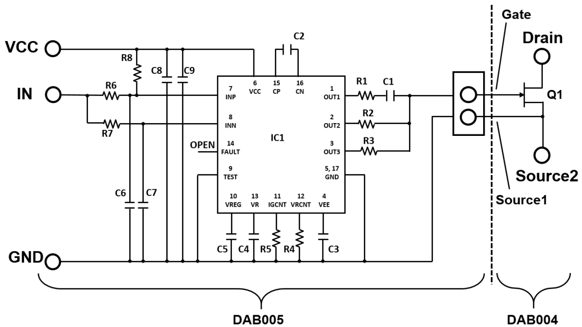
Figure 7: PGA26E07BA-DB001 schematic
