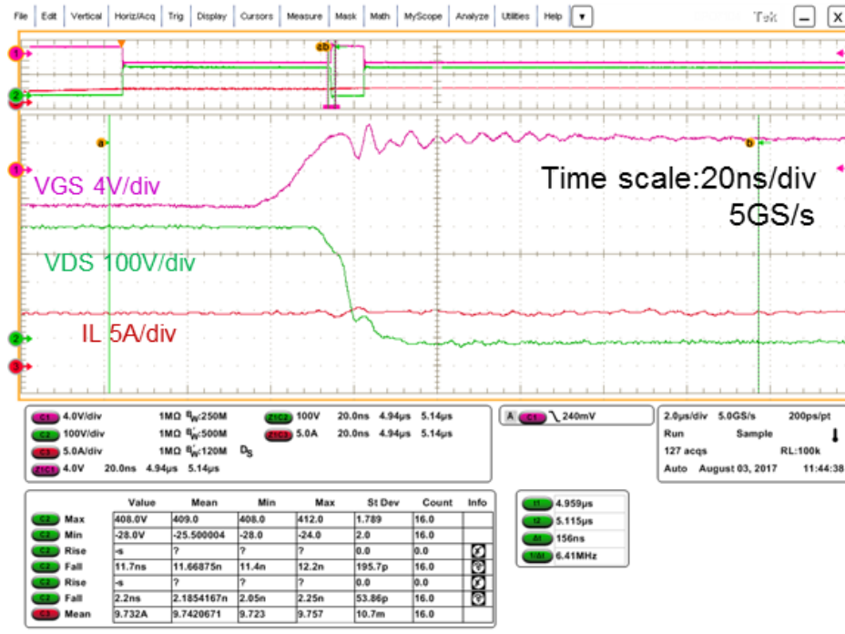
Figure 16(a): Typical turn-on waveform
