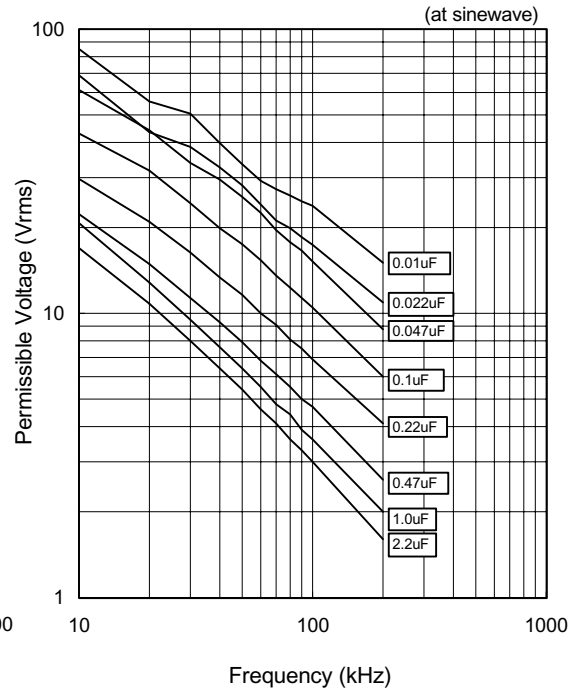
Permissible Voltage
