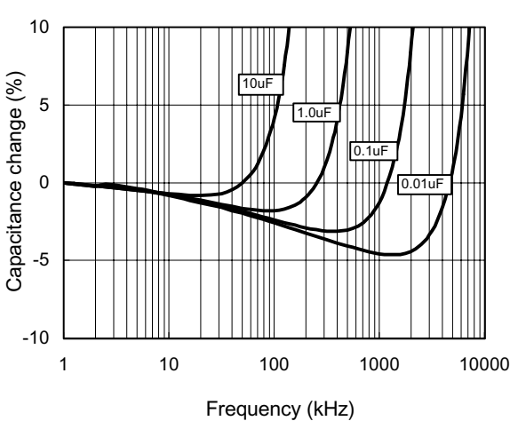
Frequency Characteristics
