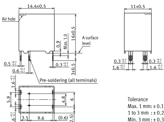
External dimensions
