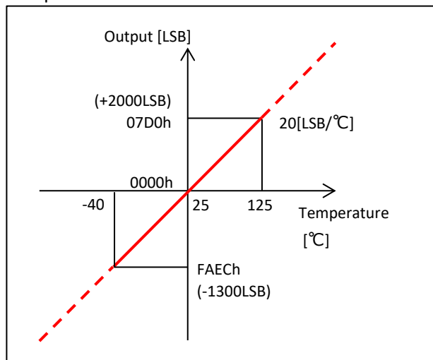
Temperature sensor
