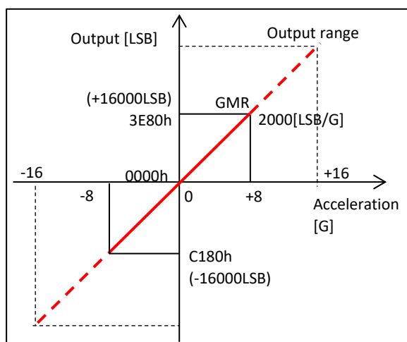
Acceleration sensor (FS: \pm 8\text{G} )
