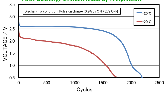
Pulse Discharge Characteristics by Temperature
