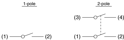
Terminal circuit diagram
