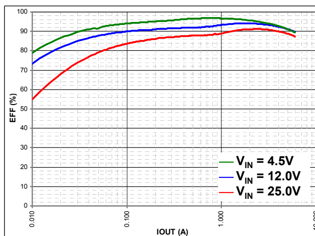
Characteristic 4-2
