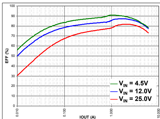
Characteristic 4-1
