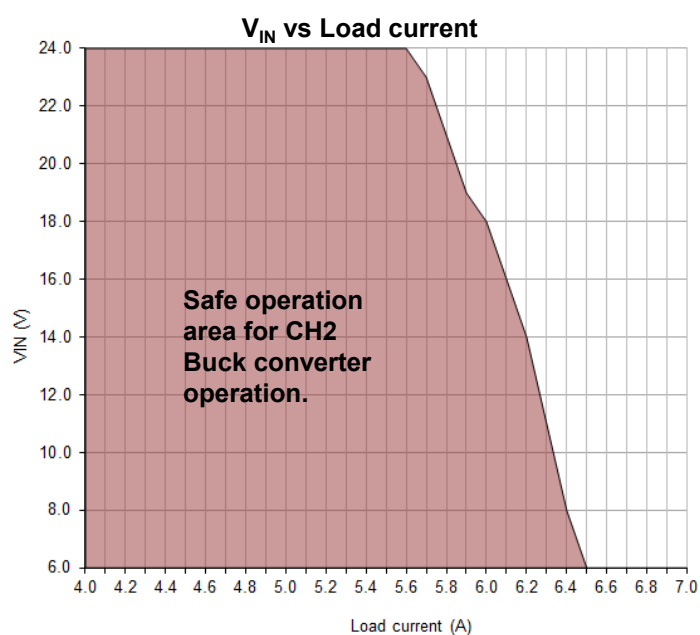
Figure 7-2 : Reference Safe Operation Area
