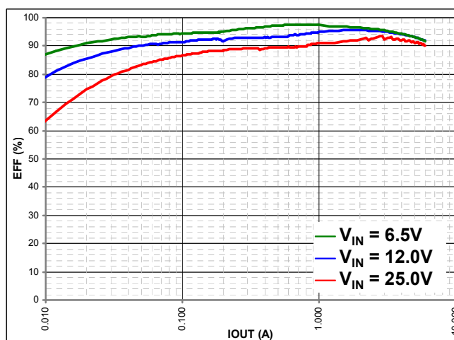
Characteristic 4-3
