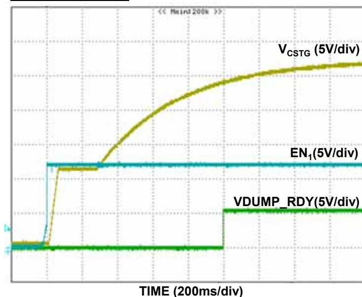
Characteristic 1-1
