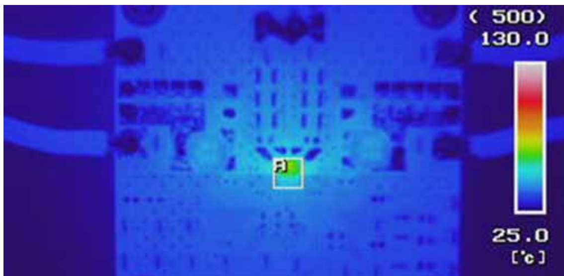
Figure 7-1 : Thermal image
