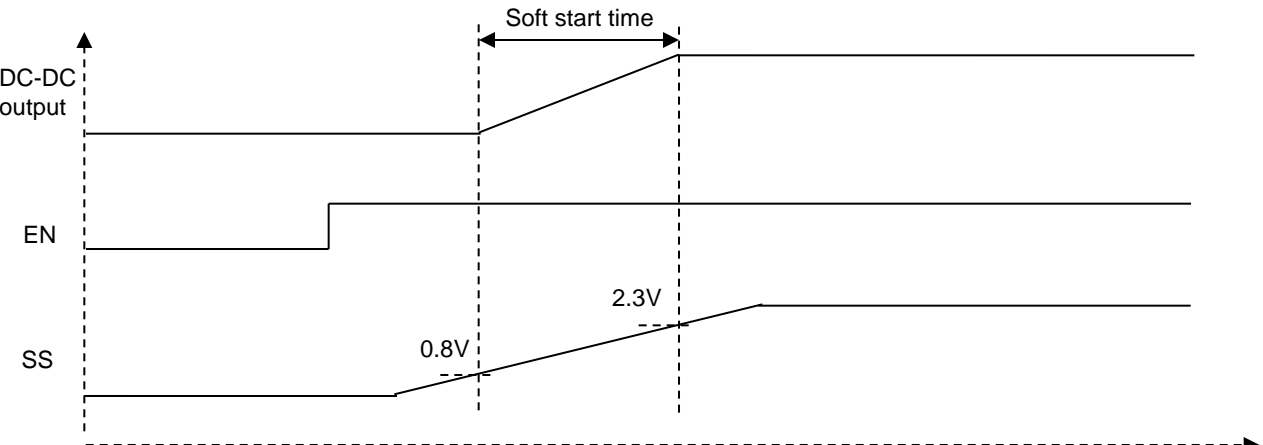
Figure : Soft start operation timing chart
