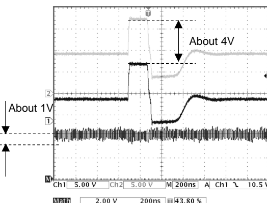
Figure : BT waveform, LX waveform, BT-LX voltage (with 330Ω condition)
