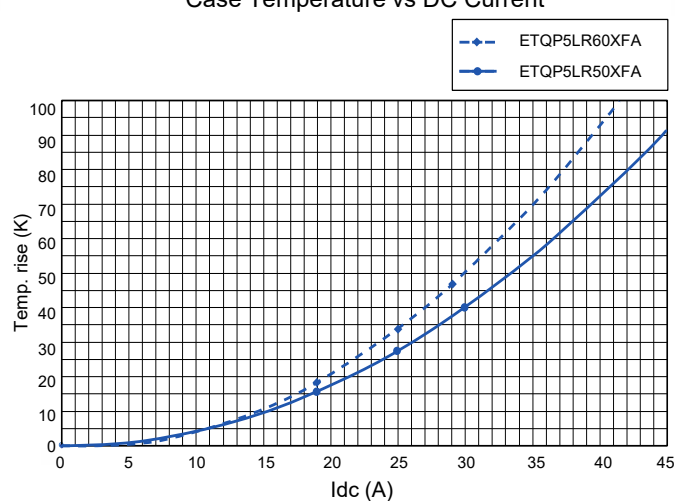
Case Temperature vs DC Current
