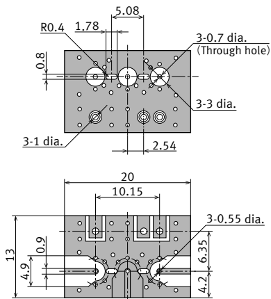
Calibration board
