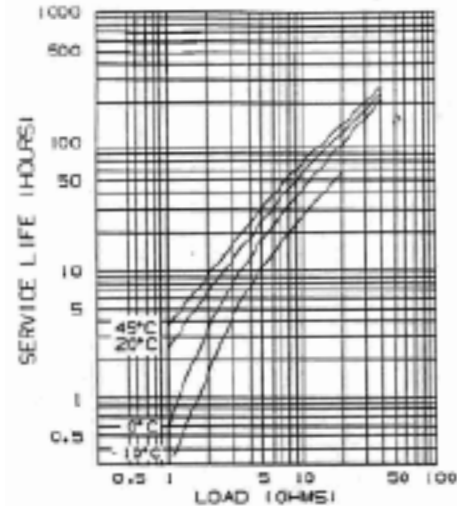
Typical Temperature Characteristics 0.9 Volts Cutoff Voltage
