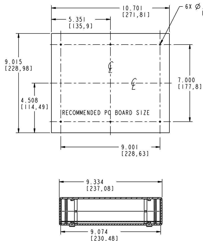
SECTION B-B
