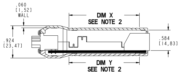
SECTION C-C
