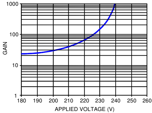
Fig. 1: APD GAIN vs BIAS VOLTAGE
