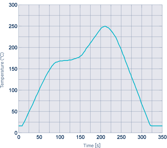
Reflow soldering profile (10)
