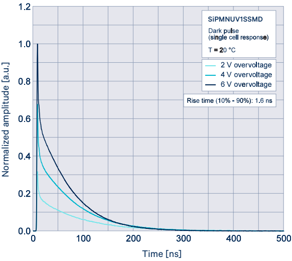
Pulse shape at different overvoltage (recharge time constant is 70 ns)
