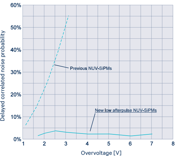
Delayed correlated noise probability (delayed crosstalk and afterpulse)
