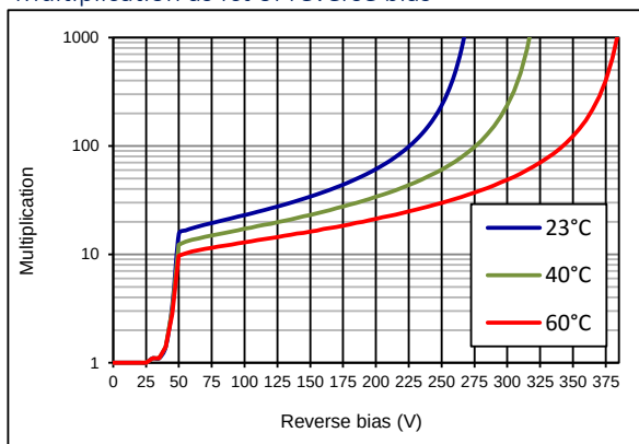
Multiplication as fct of reverse bias
