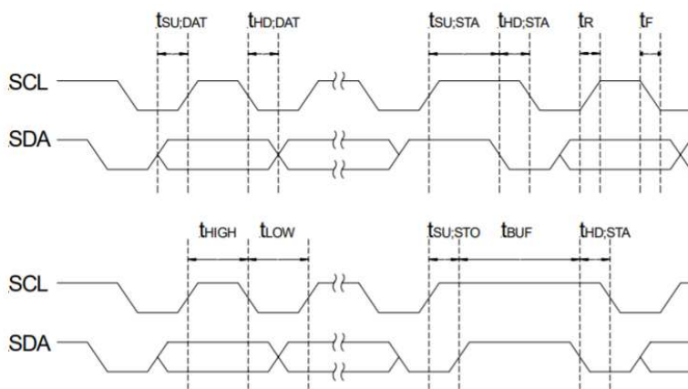
Fig. 2: Timing characteristics
