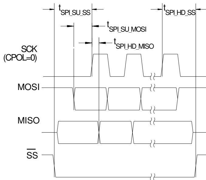
Fig. 3: Timing characteristics
