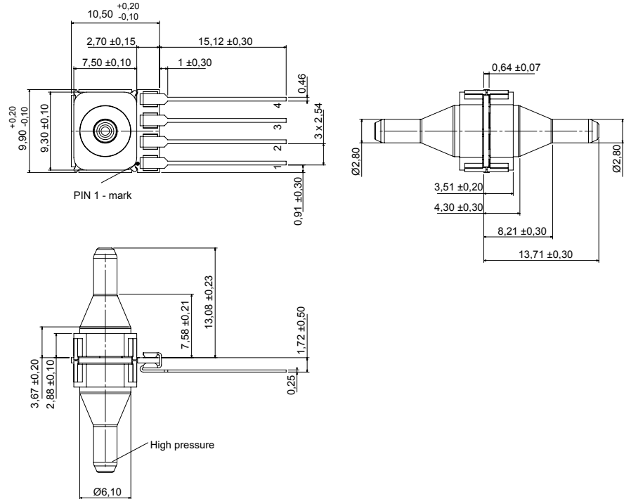
HMU...DU5... (SIL, 2 ports axial opposite side, needle big)
