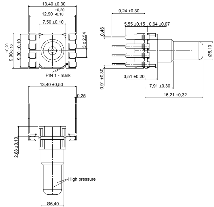
HMA...Z6... (DIP, 1 port axial, straight big)
