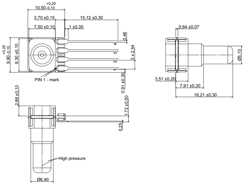
HMA...X6... (SIL, 1 port axial, straight big)
